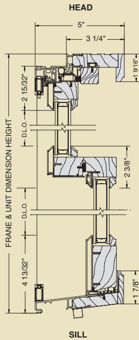
Vertical Section
